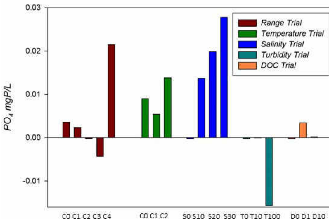
Figure 7. Global summary of difference between instrument and reference measurements for all laboratory tests at each trial conditions for the Systea-PO4 analyzer.
