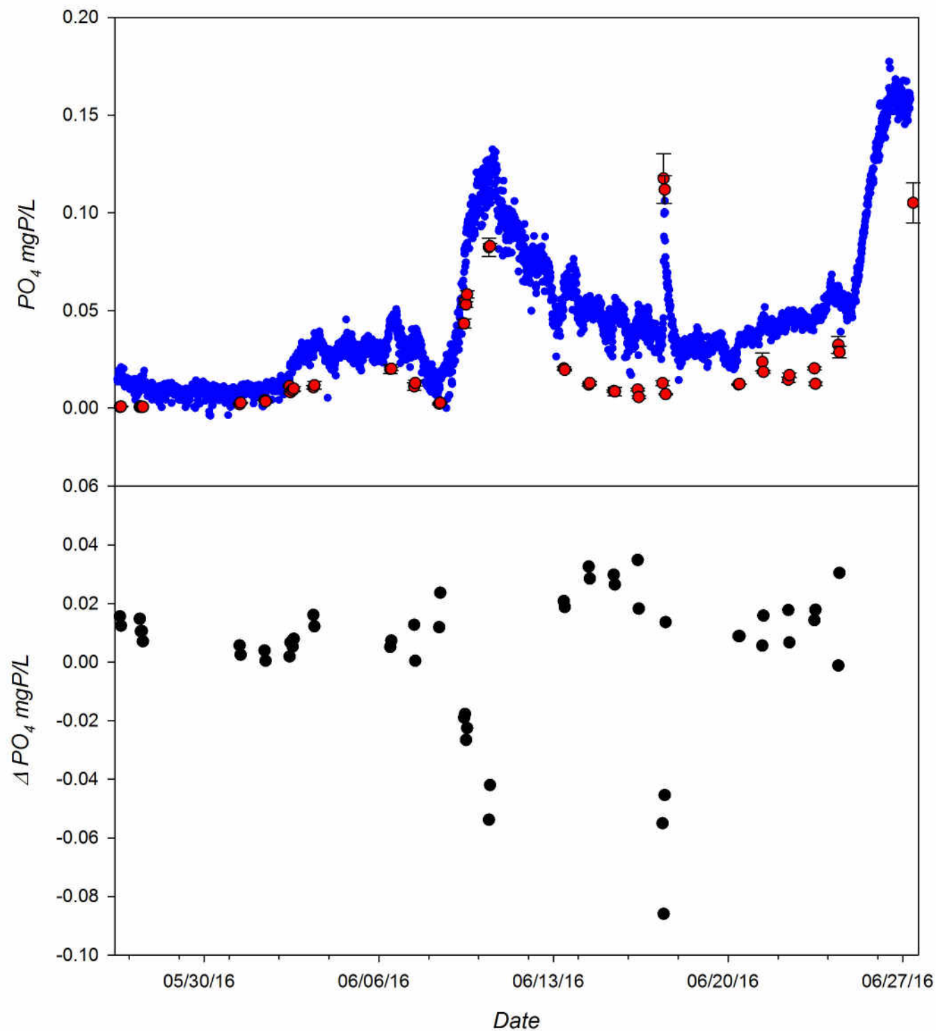
Figure 10. Top Panel: Time series plot of the Systea-PO4 measurement (blue dots) and reference measurements (red dots) of phosphate in mgP/L. Bottom Panel: Time series plot of the difference between the Systea-PO4 and reference measurements of phosphate in mgP/L (instrument – reference) during the freshwater deployment in the Maumee River at Waterville, OH.
