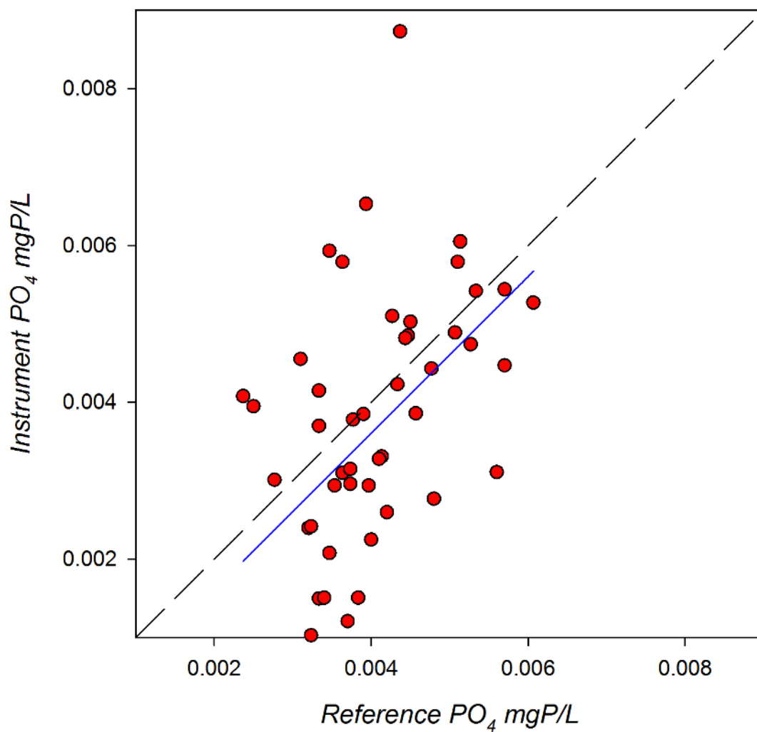
Figure 21. HIMB field response plot of Systea- PO_4 compared to reference PO_4 samples. The plotted line represents a 1:1 correspondence, the blue line represents the linear regression.
