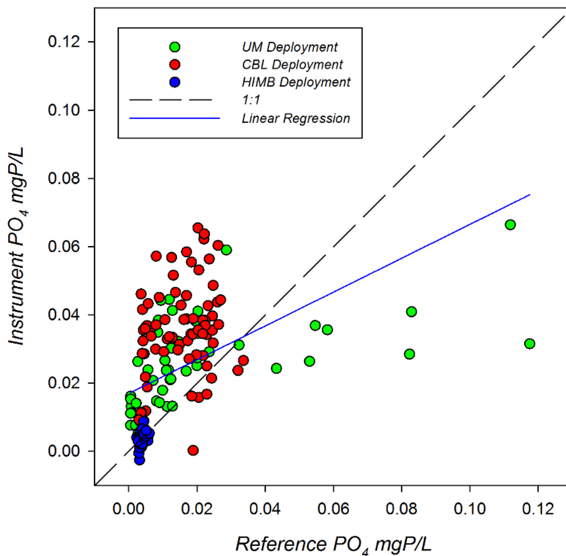
Figure 23. Global response plot for the Syssta-PO 4 observed during the three ACT field trials. Black dotted line represents a 1:1 correspondence, the blue line represents the linear regression.
