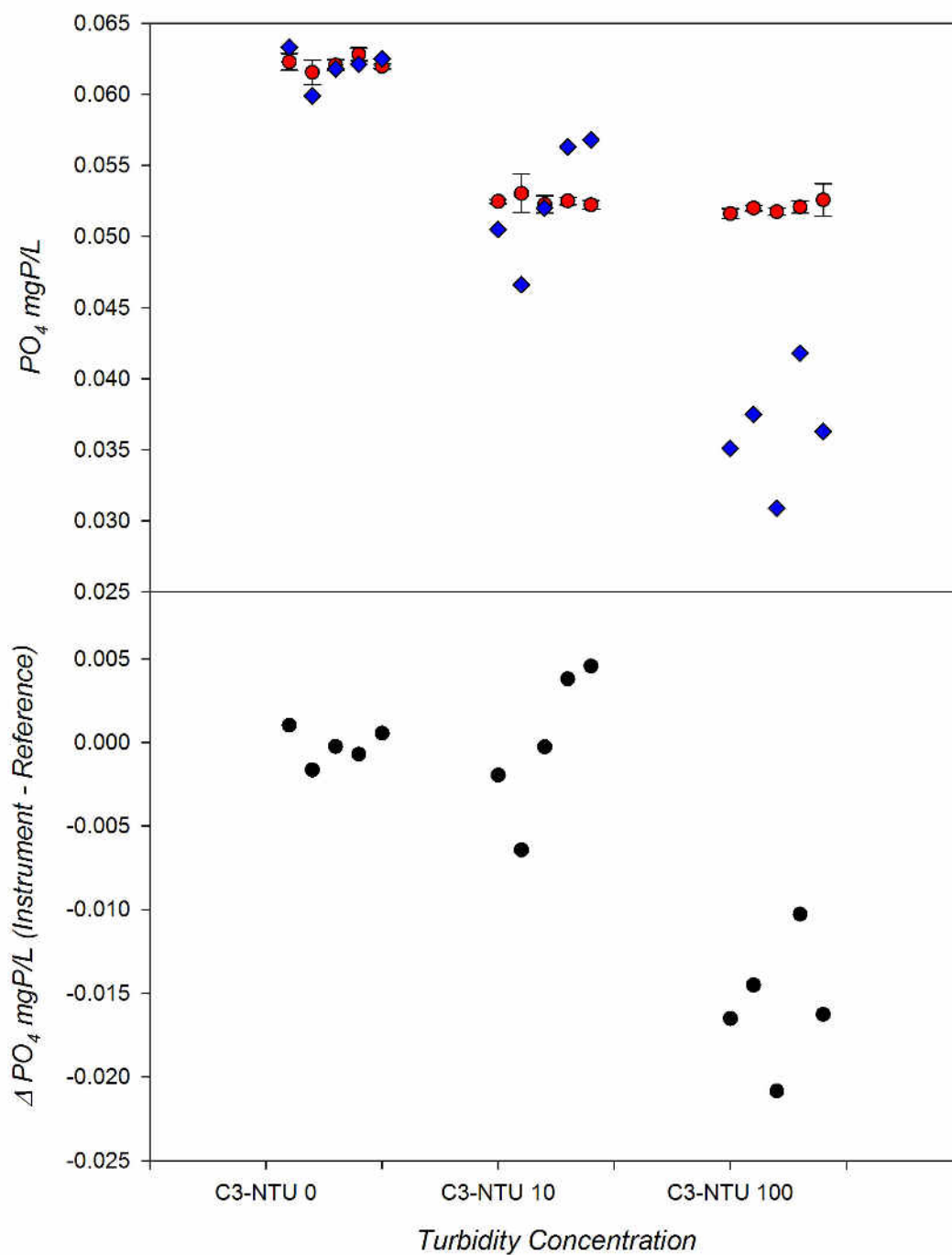
Figure 5. Top Panel: Plot of instrument (blue dots) and reference (red dots) measurements of PO 4 (mgP/L) at three turbidity levels for the C3 concentration. Five replicate measurements were made at each concentration level. Bottom Panel: Plot of the absolute difference between Syssta-PO4 and reference measurement.
