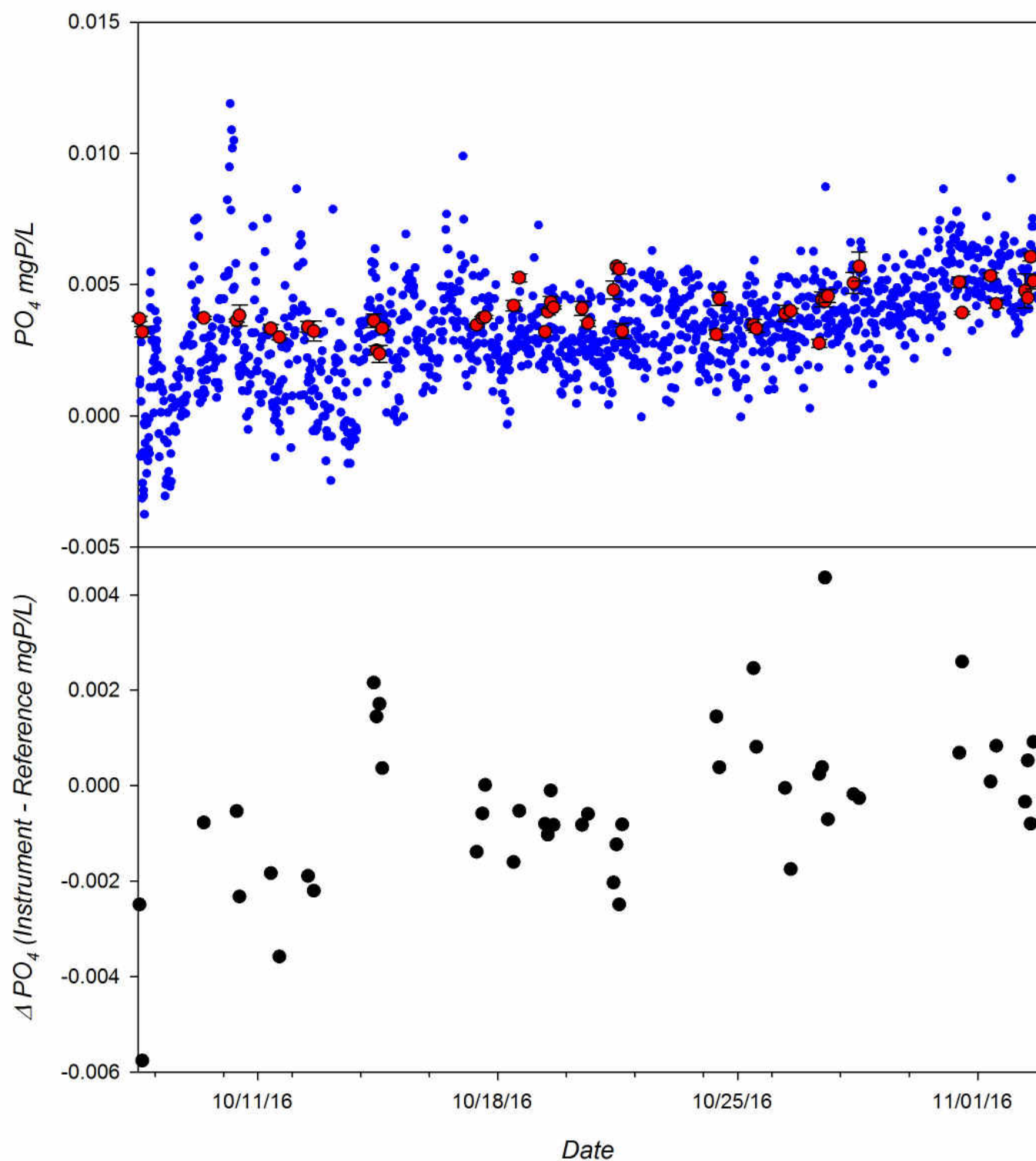
Figure 20. Top panel: Time series of PO_4 measured by the Systea- PO_4 deployed during the one month HIMB field trial. Continuous PO_4 recordings from instrument (blue dots) and PO_4 of adjacent grab samples (red circles.) Bottom Panel: Time series of the difference between the Systea- PO_4 and reference measurements for each matched pair (Instrument mgP/L – Reference mgP/L).
