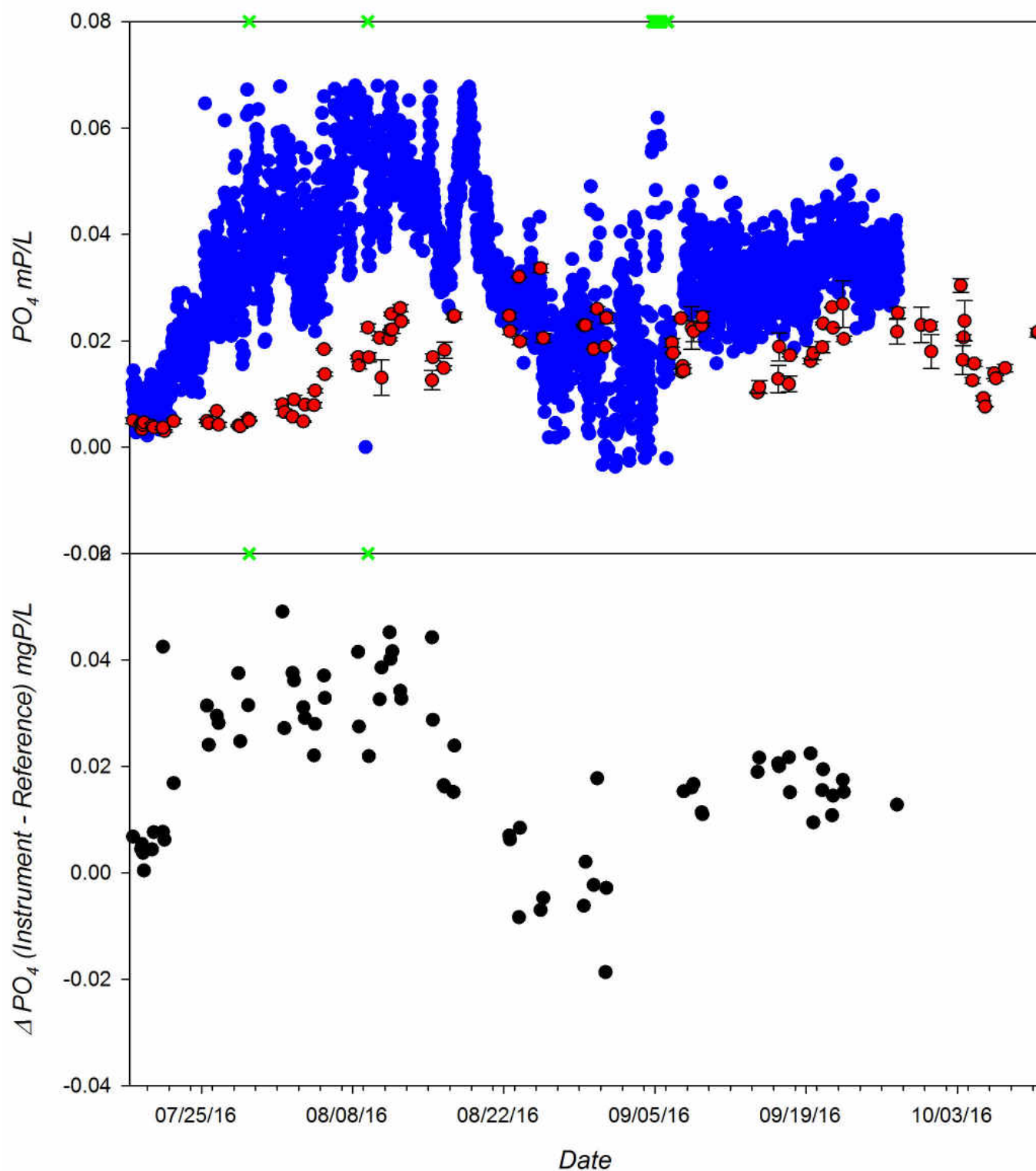
Figure 15. Time series of \text{PO}_4 measured by the Syste-a- \text{PO}_4 during the 84 day CBL field trial. Top Panel: Continuous \text{PO}_4 recordings from instrument (blue circles) and \text{PO}_4 of adjacent grab samples (red circles). Bottom Panel: The difference in measured \text{PO}_4 relative to reference samples (Instrument mgP/L – Reference mgP/L) observed during deployment.
