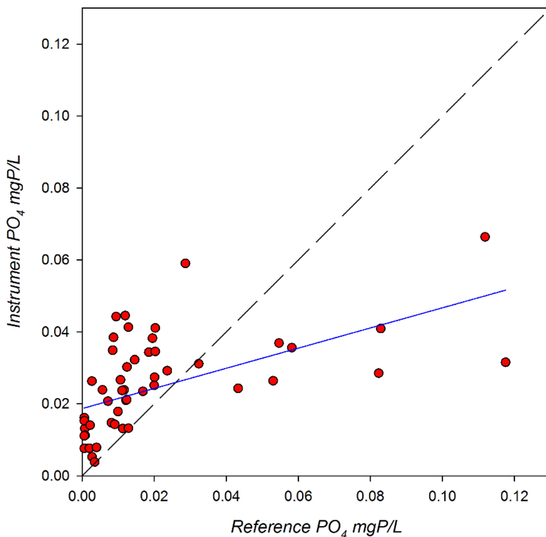
Figure 11. Maumee River field response plot for the 32 day deployment of the Systea-PO4 compared to reference PO 4 samples. The plotted line represents a 1:1 correspondence, the blue line represents the linear regression.
