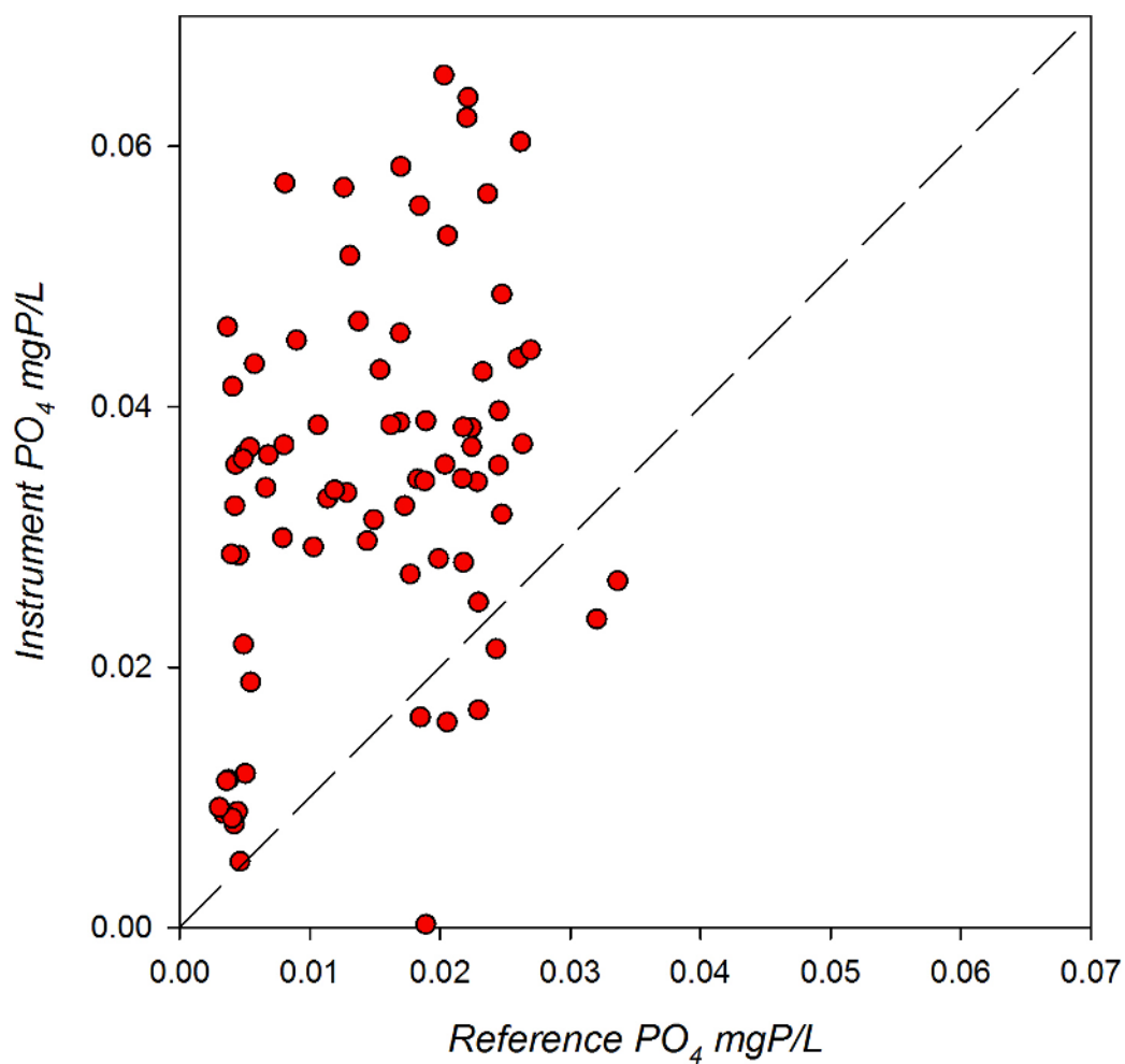
Figure 16. CBL field response plot for Systea-PO4 compared to reference PO_4 samples. The plotted line represents a 1:1 correspondence.
