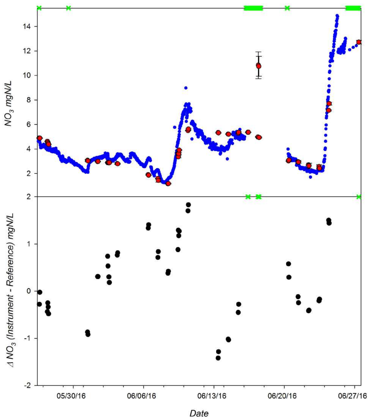
Figure 10. Top Panel: Time series plot of the Systea- \text{NO}_3 measurement (blue dots) and reference measurements (red dots) of nitrate in mgN/L. The green crosses at the top of figure represent flagged data (not values) and are plotted on the date of occurrence. Bottom Panel: Time series plot of the difference between the Systea- \text{NO}_3 and reference measurements of nitrate in mgN/L (instrument – reference) during the freshwater deployment in the Maumee River at Waterville, OH.
