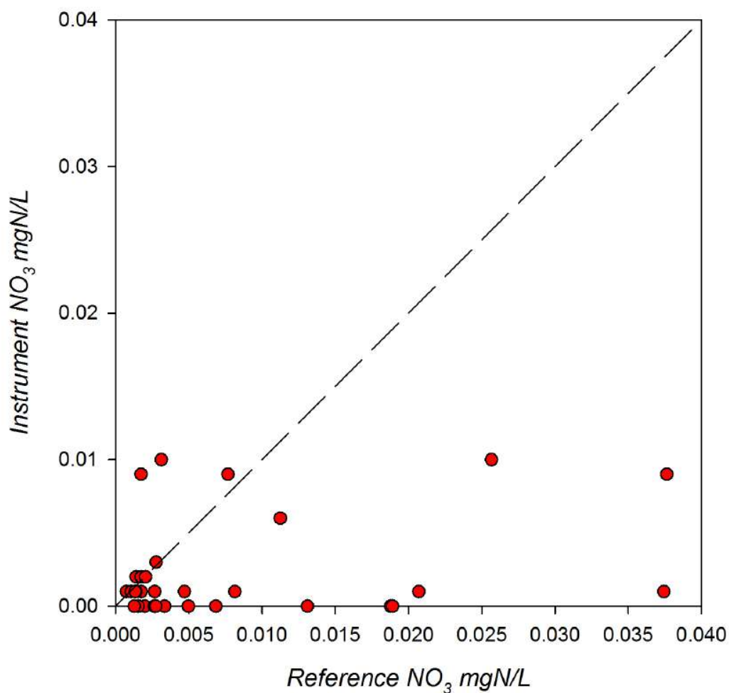
Figure 16. CBL field response plot for Syssta-NO 3 compared to reference NO 3 samples. The plotted line represents a 1:1 correspondence.
